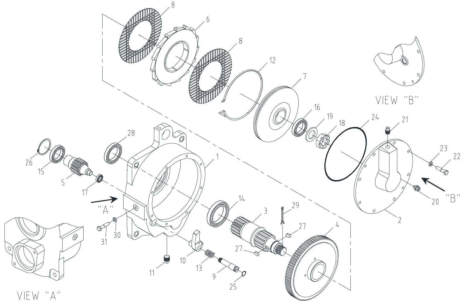
Fig. 2-1 SCS886 WINCH R/ G ASS'Y
