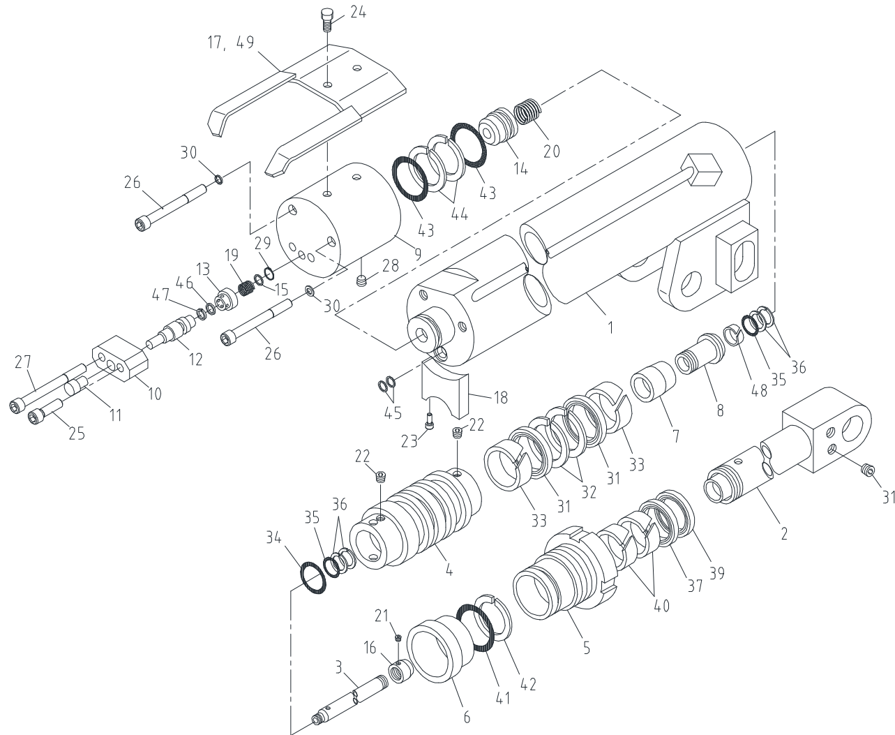
Fig. 1 -1 -1 SCS886 TELESCOPIC CYL'(1st) ASS'Y
